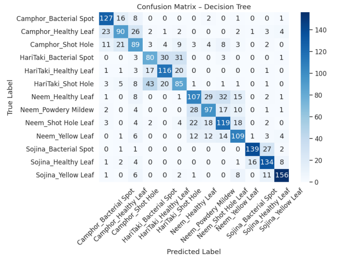
Fig. 11. Confusion matrix on the test set using an Decision Tree classifier trained on MoCo V3 features.
